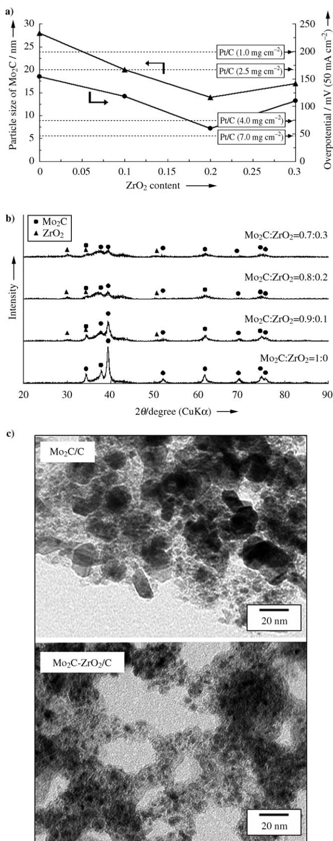
Figure 2. a) Particle size of \text{Mo}_2\text{C} and overpotential of \text{Mo}_2\text{C}-\text{ZrO}_2/\text{C} for propane oxidation as a function of \text{ZrO}_2 content in \text{Mo}_2\text{C}-\text{ZrO}_2/\text{C} . The overpotential of the \text{Mo}_2\text{C}-\text{ZrO}_2/\text{C} anode was measured under the same conditions as in Figure 1. b) XRD patterns of \text{Mo}_2\text{C}-\text{ZrO}_2/\text{C} with different proportions of \text{ZrO}_2 . c) TEM micrographs of \text{Mo}_2\text{C}/\text{C} and \text{Mo}_2\text{C}-\text{ZrO}_2/\text{C} ( \text{Mo}_2\text{C}:\text{ZrO}_2 = 0.8:0.2 ).
